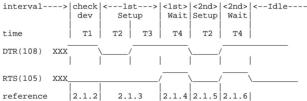
Figure 1 - Example COM Enumerator External Timing Diagram
